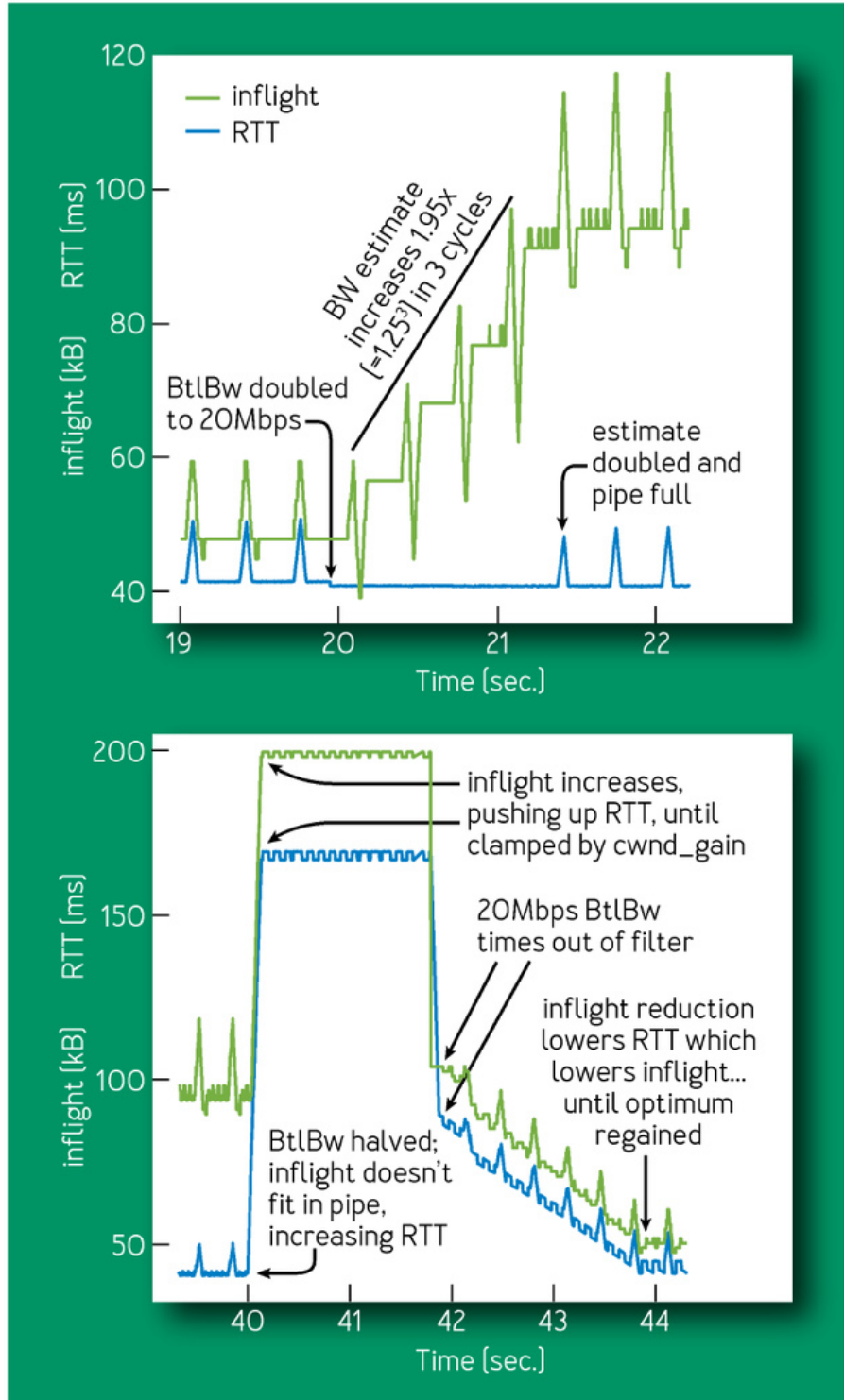
FIGURE 3: BANDWIDTH CHANGE
