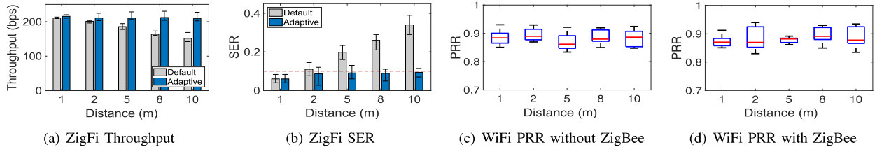
Fig. 16. ZigFi performance under different distance between the ZigBee sender and the WiFi receiver in the NLOS scenario.
