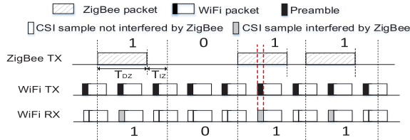
Fig. 6. The basic communication scheme of ZigFi.
