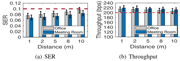
Fig. 17. ZigFi performance in different environments.
