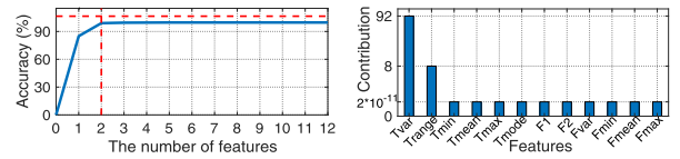
(a) SVM accuracy with the increase of features (b) The contribution rate of twelve features
