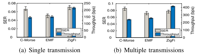
Fig. 14. Performance comparison of C-Morse, EMF, and ZigFi.
