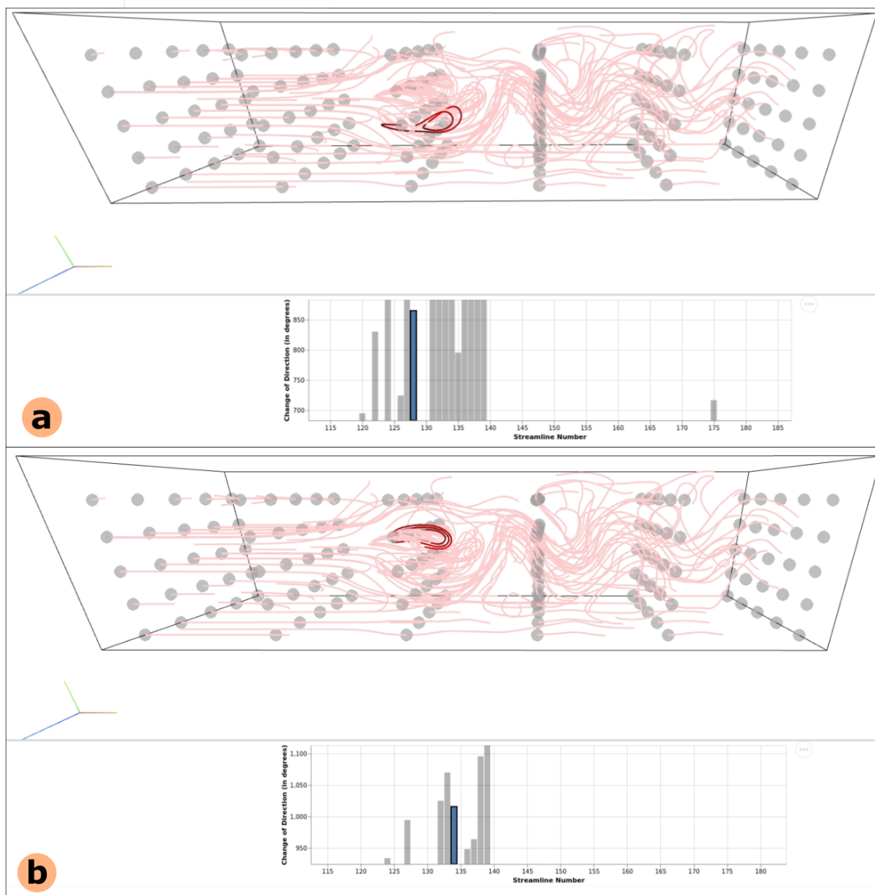
Figure 6. Two examples of the interaction between the Vega-Lite plot and the 3D view. (a) and (b) each shows the highlighted streamline whose index is the selected bar entry on the Vega-Lite plot.
