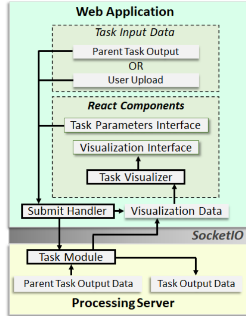
Figure 3. User Task Creation and Modification.
