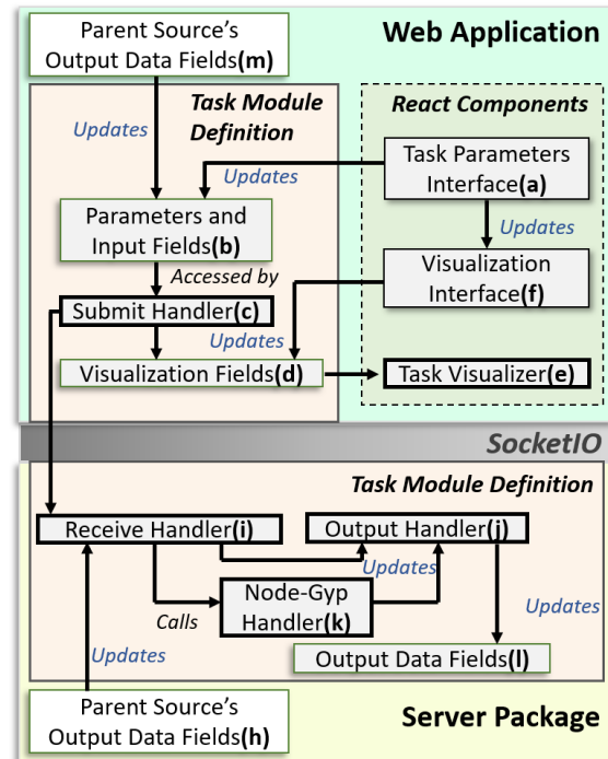
Figure 2. The main components of an FCLWebVis Task. They are required to include a new task.
