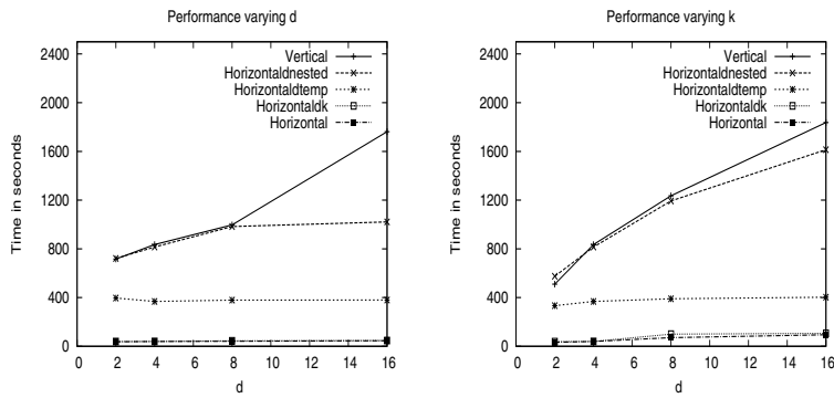
Figure 1. Query optimizations for distance computation: Varying d and k ; defaults d = 4, k = 4, m = 2, n = 1M .
