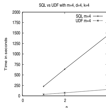
Figure 4. Distance computation for classification: SQL vs UDF: Time growth varying n for m=4 ; defaults d = 4, k = 4, n = 1M .
