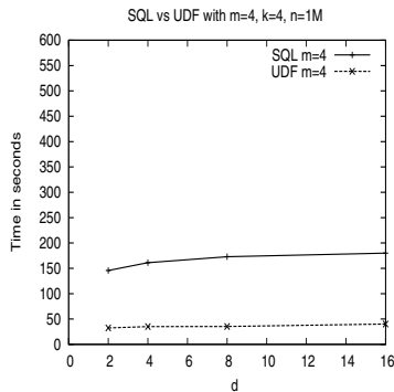
Figure 5. Distance computation for classification: SQL vs UDF: Time growth varying d for m=4 ; defaults d = 4, k = 4, n = 1M .
