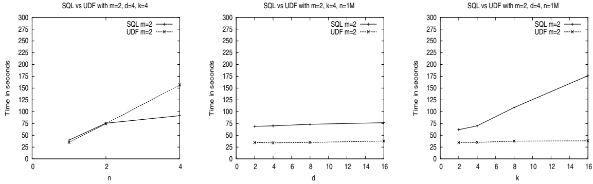
Figure 3. Distance computation for classification: SQL vs UDF: Time growth varying n , d and k for m=2 ; defaults d = 4, k = 4, n = 1M .
