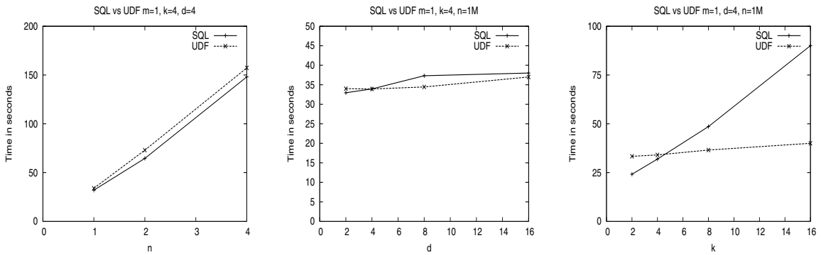
Figure 2. Distance computation for clustering: SQL vs UDF: Time growth varying n, d and k ; defaults d = 4, k = 4, n = 1M .
