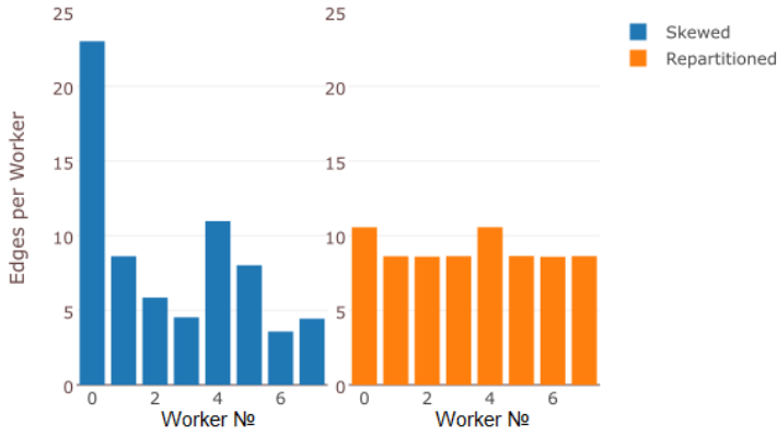
Fig. 6 Array DBMS: Living journal data set. Another perspective of the data density. Data distribution in cluster before and after repartitioning. Vertical axis shows edges per worker. Horizontal axis identifies workers.
