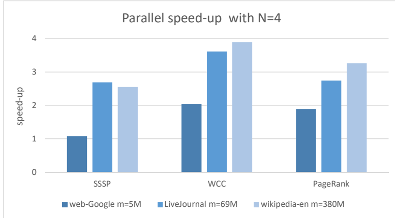
Fig. 9 Parallel speedup for SSSP, Connected Components and PageRank for 3 data sets (4 Nodes)
