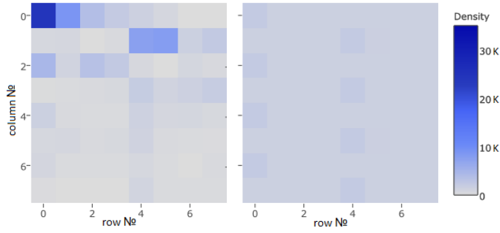
Fig. 5 Array DBMS: Living Journal data set. Adjacency matrix heat map before (left) and after (right) repartitioning. The number in the axis are coordinates identifying chunks in the disk array storage. Chunk (0,0) on the left presents the maximum density.
