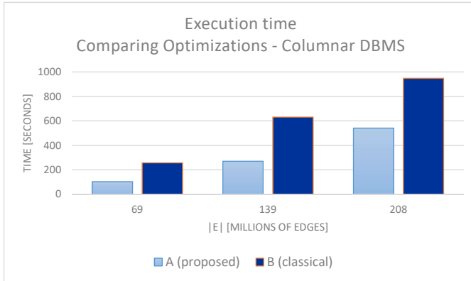
Fig. 3 Comparing execution times in columnar DBMS: (A) Proposed partition strategy. (B) Classical parallel join optimization by replication of the smaller table
