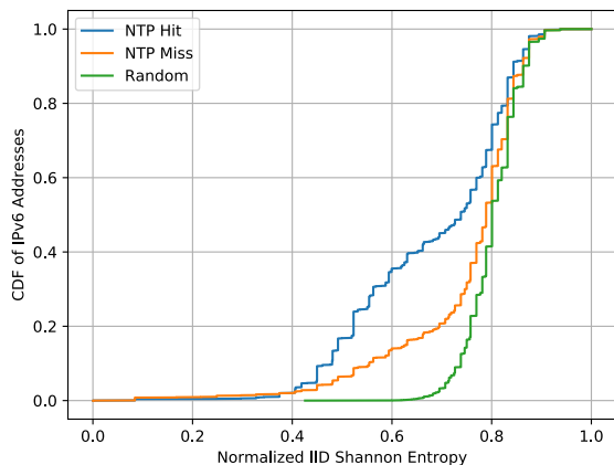
Figure 3: CDF of the IID entropy of NTP clients probed back with Yarrp and ZMap6. The clients that we passively detect from running an NTP client are responsive to back scanning, particularly those with slightly lower entropy in their IID.
