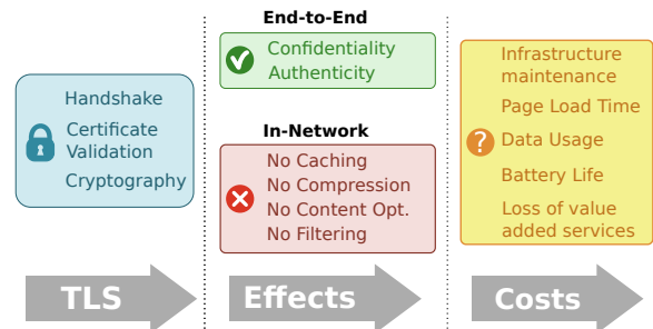
Figure 1: The HTTPS adoption impact chain.
