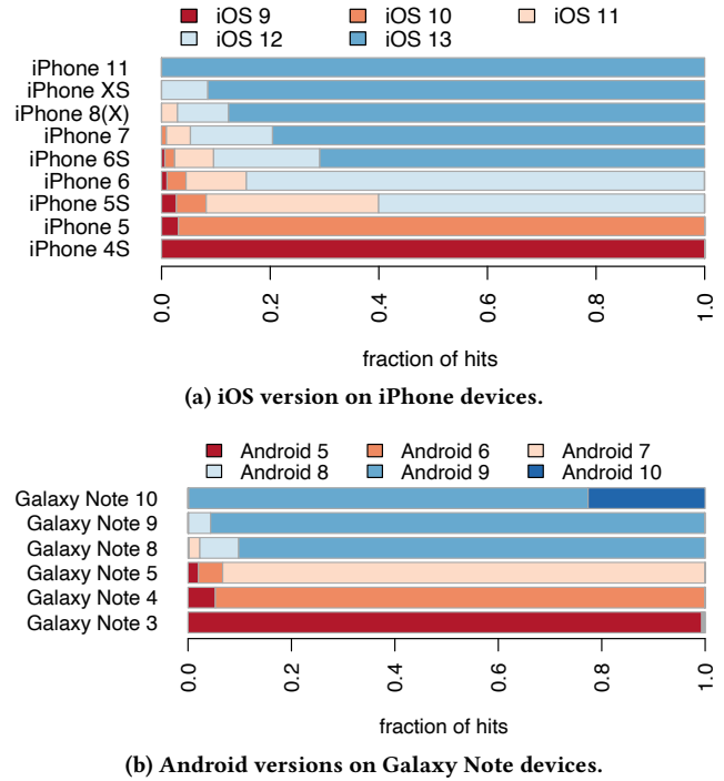
Figure 15: Fraction of requests matching a specific OS version on January 1, 2020 running on select devices. Older devices tend to run older OS versions, in part due to non-availability of OS updates for older devices, and in part due to a lack of action by users.
