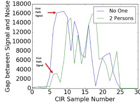
Figure 4: CIR in presence of 2 persons vs no person
