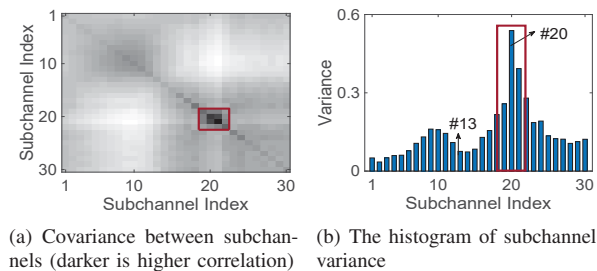
Fig. 5. The relationship among WiFi subchannels
