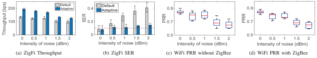
Fig. 17. ZigFi performance under different intensity of noise
