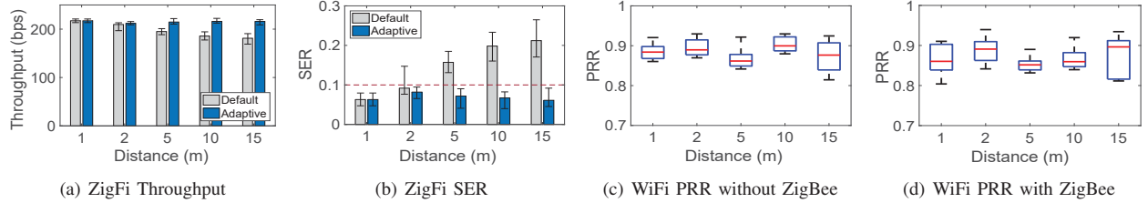
Fig. 16. ZigFi performance under different distance between the WiFi sender and the WiFi receiver
