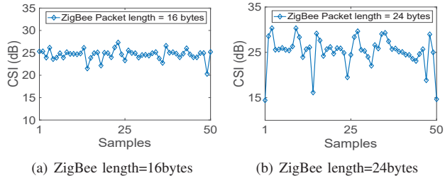
Fig. 6. The CSI sequences with different ZigBee packet lengths
