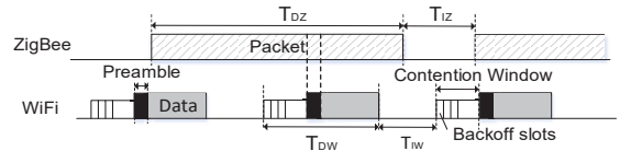
Fig. 3. Illustration of overlapping ZigBee and WiFi packets
