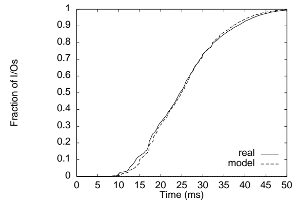
d. Final model; includes rotational position modelling and detailed disk data layout.
