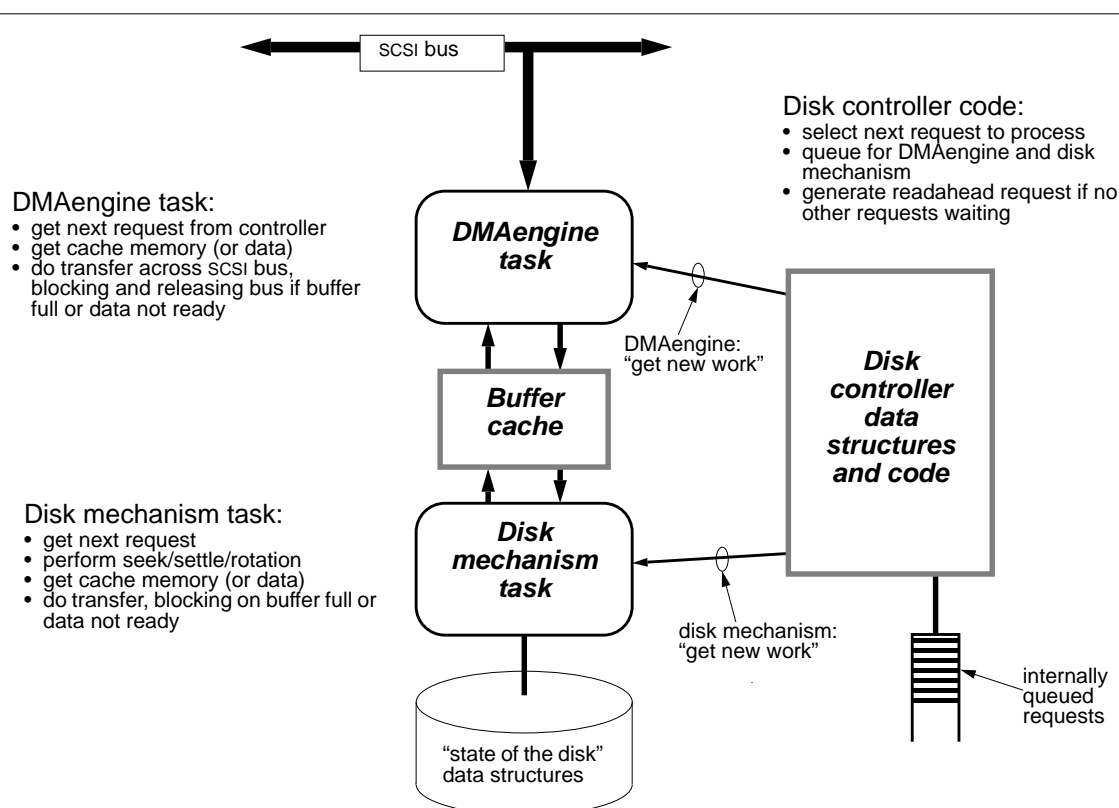
Figure 3: simulation model structure for a single disk.
