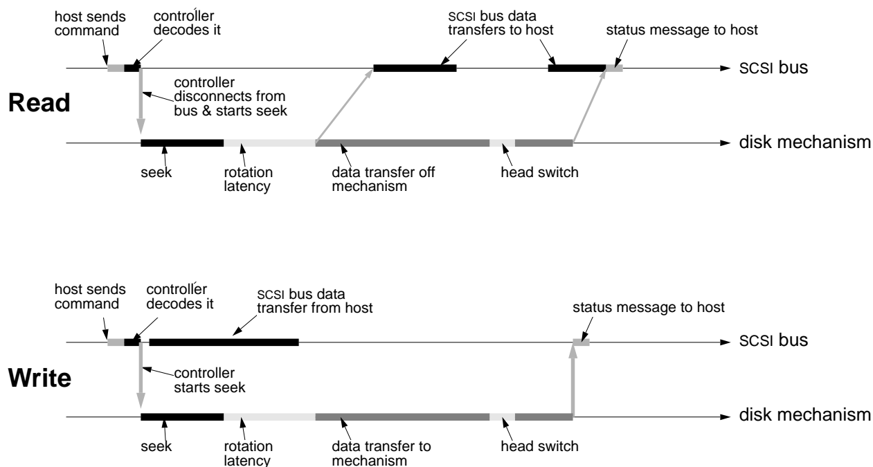
Figure 2: overlap of bus phases and mechanism activity. The low-level details of bus arbitration and selection have been elided for simplicity.
