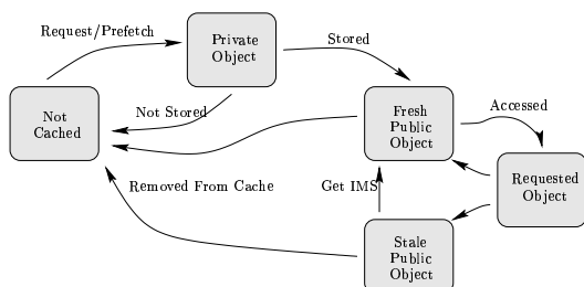
Figure 1: States of a document in a cache
