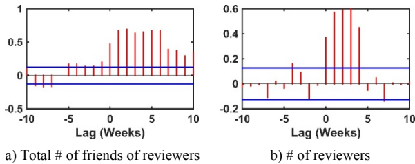
Figure 14. Truthful Popularity CCF Plot. Red lines indicate the CCF value and blue lines indicate the confidence interval bounds obtained 99% confidence ( p < 0.01 ).
