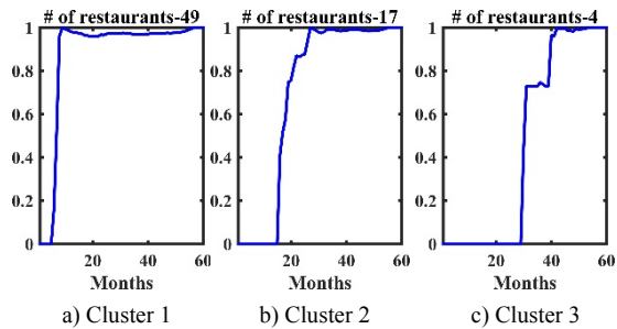
Figure 1. Time series cluster centroids with K = 3 for cumulative rating of deceptive like reviews
