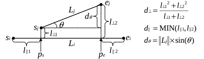
Figure 5: Three components of the distance function for line segments.
