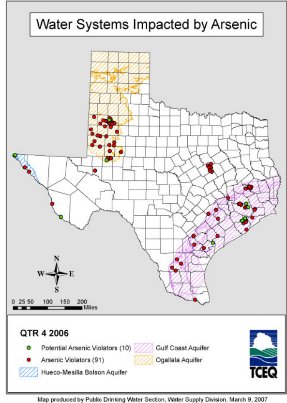
Figure 3. Arsenic pollution map (source TCEQ).
